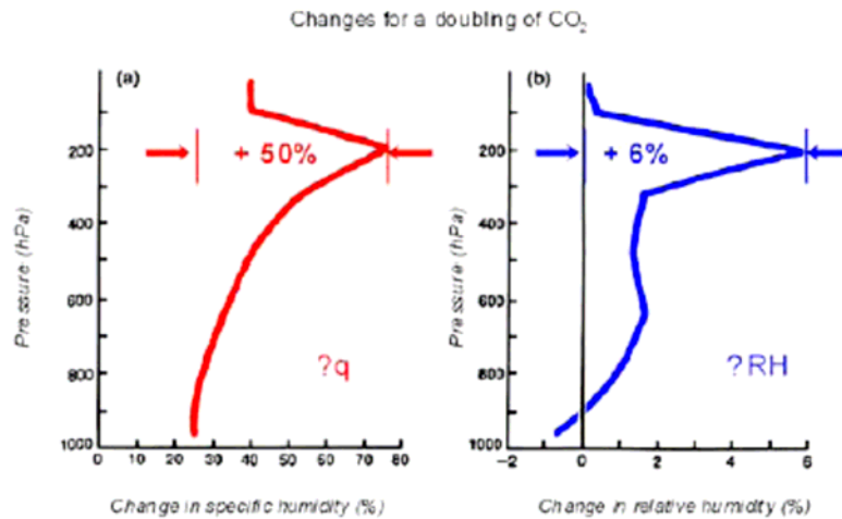
Figure 9. James Hansen's early GISS model showing his assumed increases in specific humidity (q) and RH for a doubling of CO 2 . Such water vapor assumptions are completely unrealistic, especially for conditions in the upper troposphere where water vapor typically increases less.
