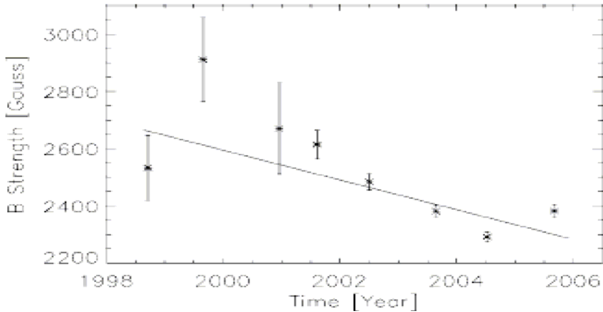
Figure 2-16: Decay in Sun's Magnetic Field since 1999
